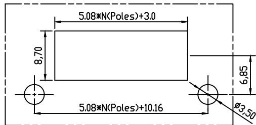
HOLE DIMENTION
