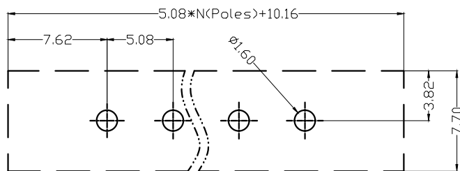
PCB Layout
