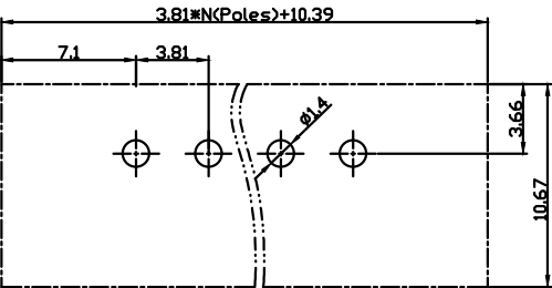
PCB LAYOUT
