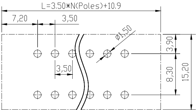
PCB Layout
