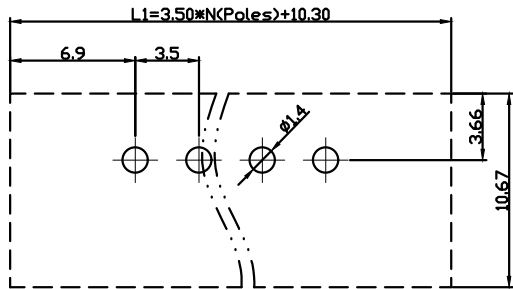
PCB LAYOUT
