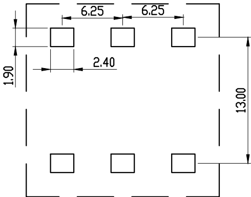
PCB LAYOUT
