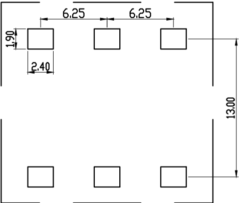
PCB LAYOUT
