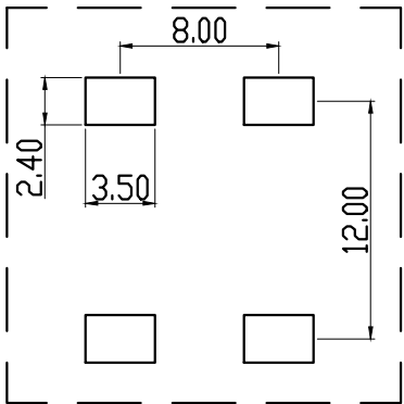
PCB LAYOUT
