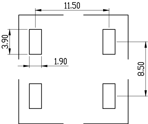
PCB LAYOUT
