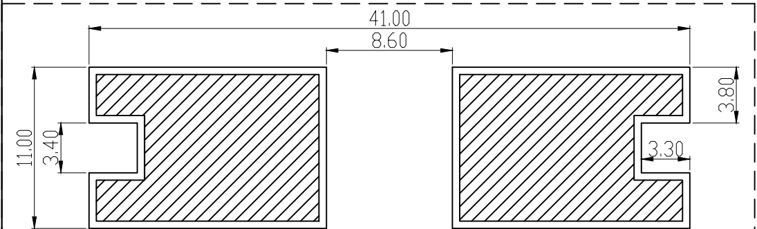
PCB layout
