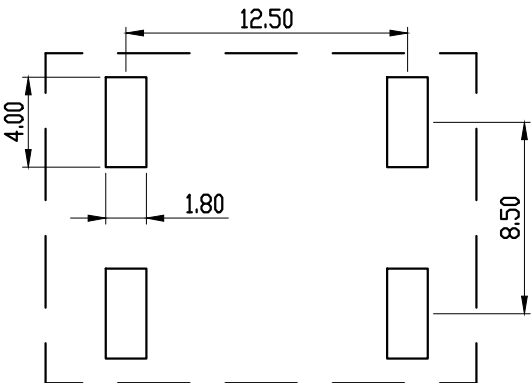
PCB LAYOUT
