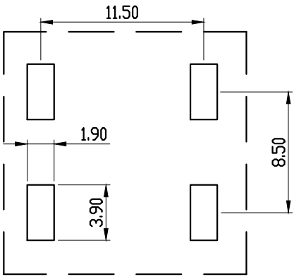
PCB LAYOUT
