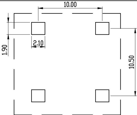
PCB LAYOUT
