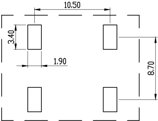
PCB LAYOUT
