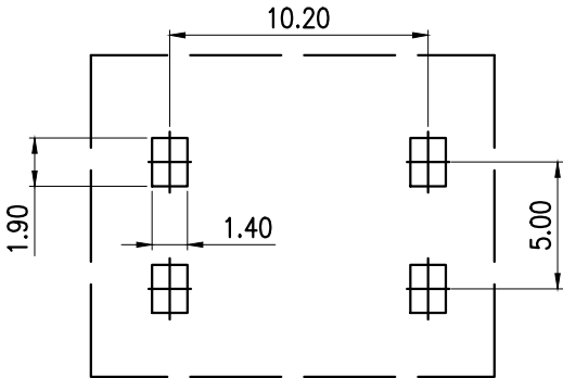
PCB LAYOUT
