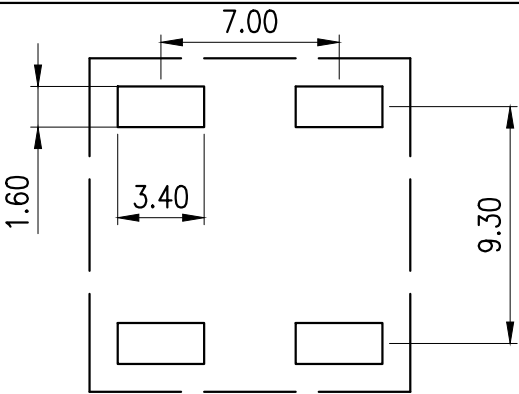
PCB LAYOUT
