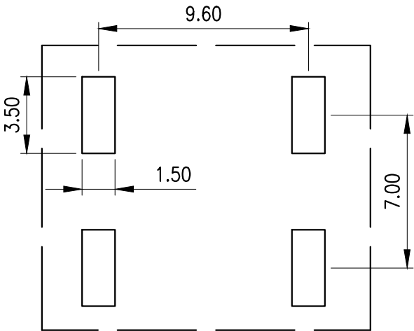
PCB LAYOUT
