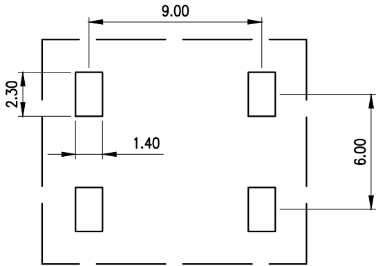
PCB LAYOUT
