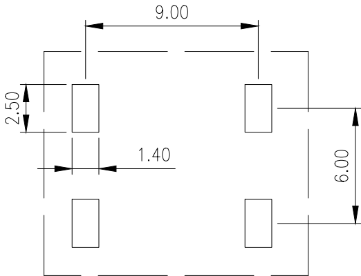
PCB LAYOUT
