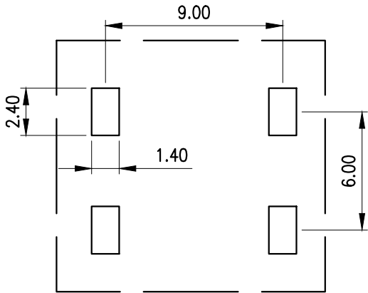
PCB LAYOUT
