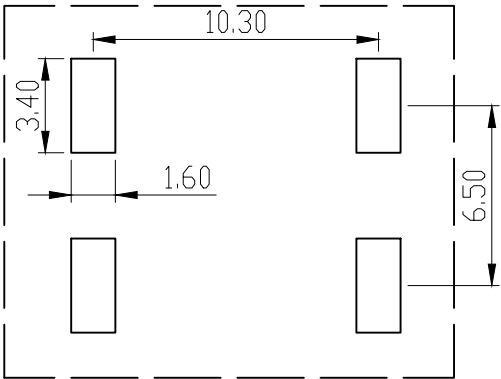
PCB LAYOUT
