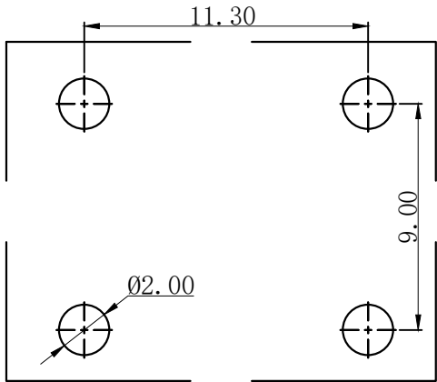
PCB LAYOUT
