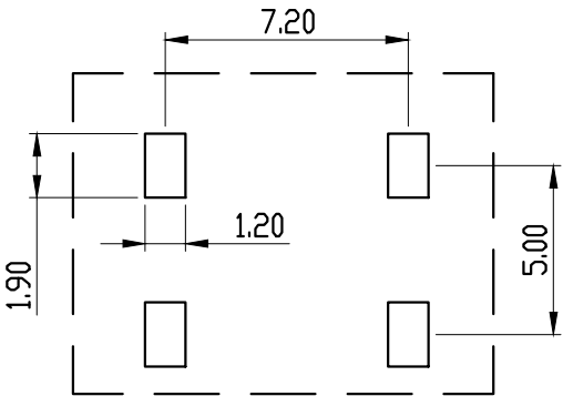
PCB LAYOUT
