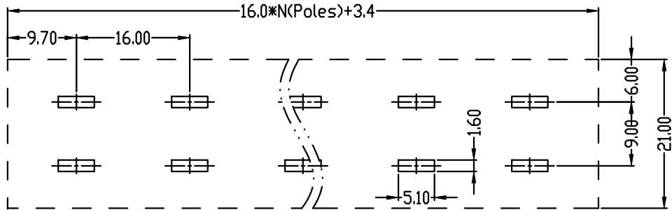
PCB Layout
