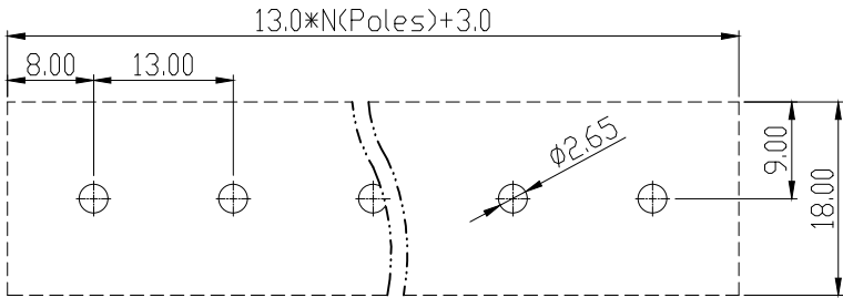
PCB LAYOUT
