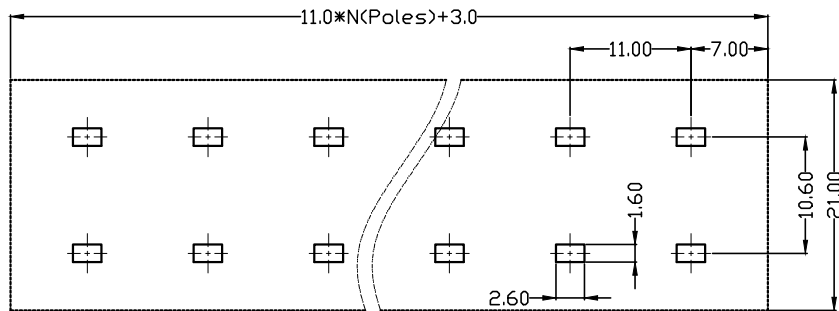
PCB Layout
