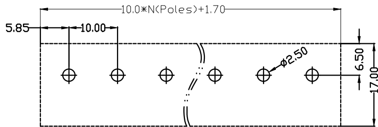
PCB LAYOUT
