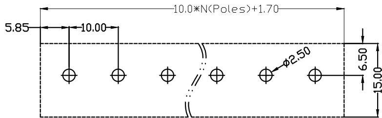
PCB LAYOUT
