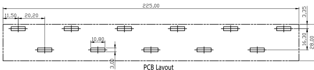
PCB Layout
