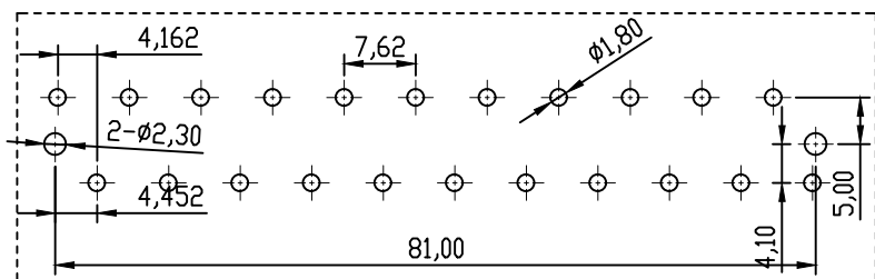
PCB LAYOUT
